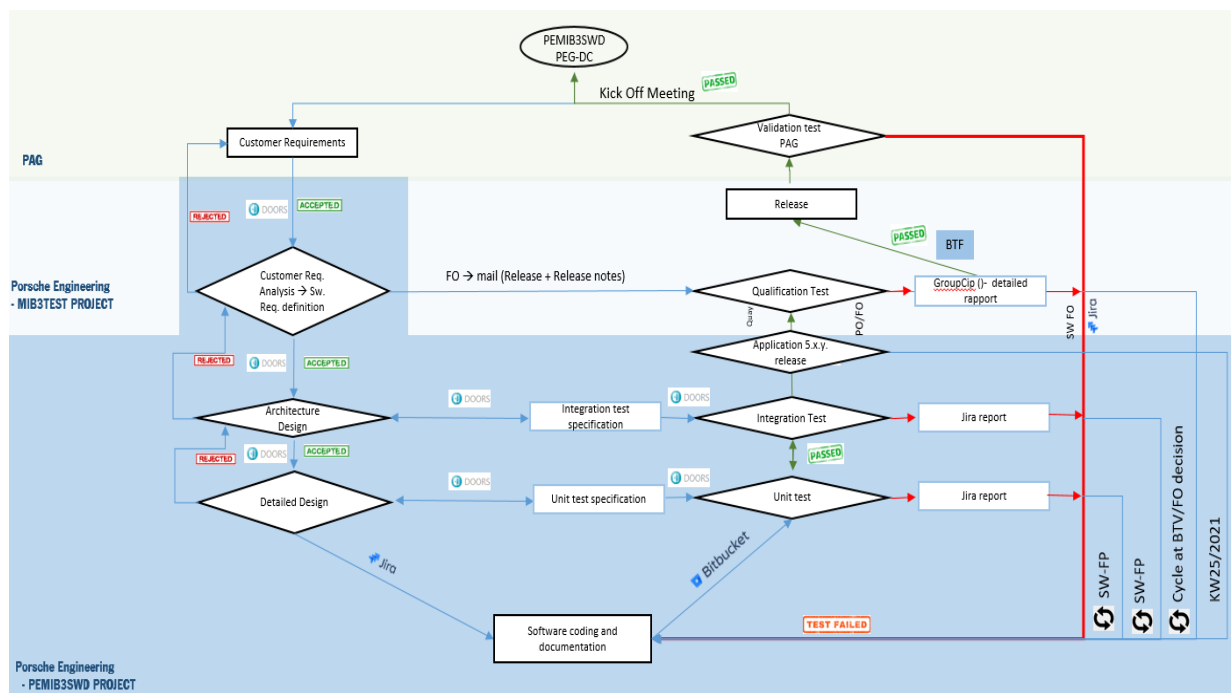
Figure 6. Development workflow for a software component used in the infotainment system
